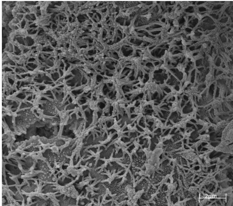
Scanning Electron Micrograph (SEM) of microvilli formation in Caco-2 culture
